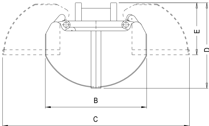
SIDE VIEW - CLOSED (DASHED LINES - OPEN)
